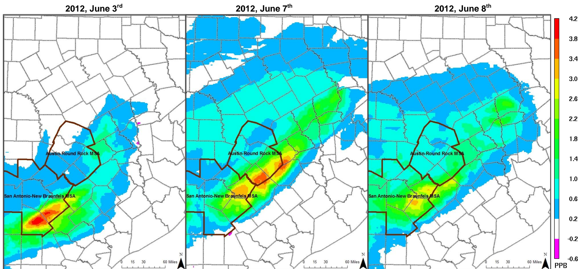
Figure 6-2: Predicted Daily Maximum Difference in 8-hour Ozone Concentrations in the 4-km Subdomain, 2012 Eagle Ford - Base Case
