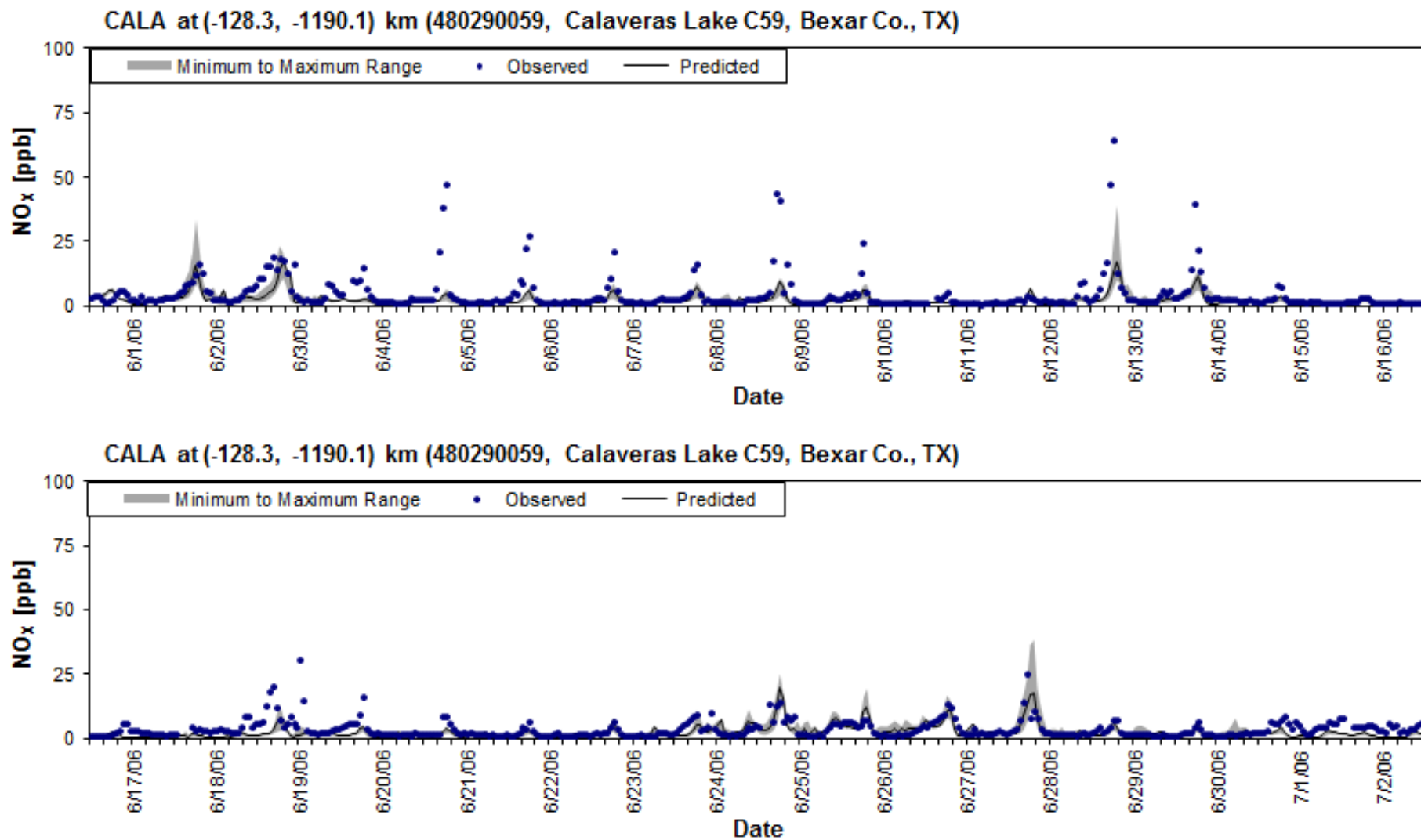
Figure 5-13: 1-Hour NO x Time Series Observed (C59) v. Predicted (CAMx) for WRF AACOG Base Case Run 3, 2006
